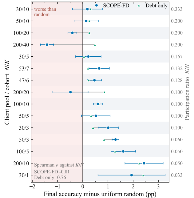
Fig. 7. Final accuracy relative to uniform random selection on FMNIST at \alpha = 0.5 , for every matched configuration, ordered by participation ratio. Each row pairs the complete score with the debt-only variant on the same seeds, the grey connector being the distance between them. Whiskers are one standard deviation of the paired difference over seeds, five per configuration except at 30/1, 30/3 and 30/10, where three are used.
